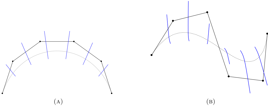
FIGURE 8. a_2 -curves with -1 < \bar{a}_2 < 2 for six equidistant t \in [0, 1] , ordinary Bézier curves dotted
