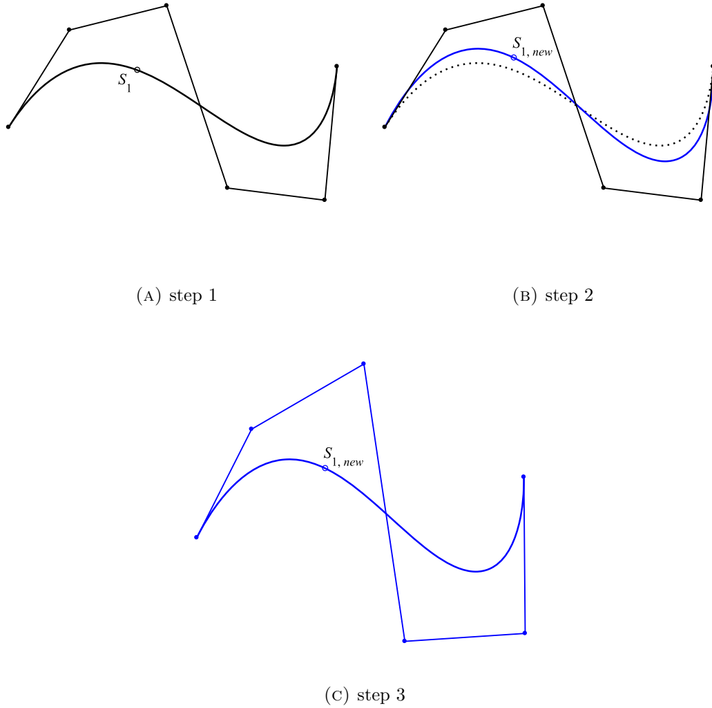
FIGURE 7. Illustration of the three steps of the proposed design method
