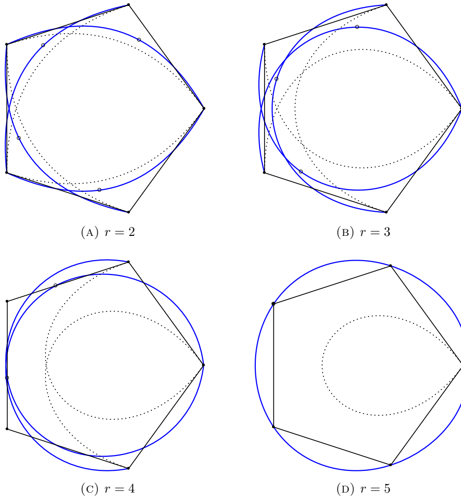
FIGURE 5. (Intermediary) generalized Bézier curves \mathbf{x}_k^r for \bar{a} = (1, -1/5, 2/25, -6/125, 24/625) with points \mathbf{b}_k^r for t = .4 , ordinary Bézier curves dotted
